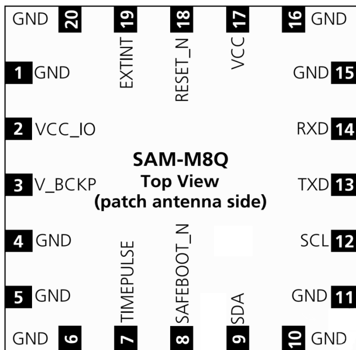
Figure 2: Pin Assignment
